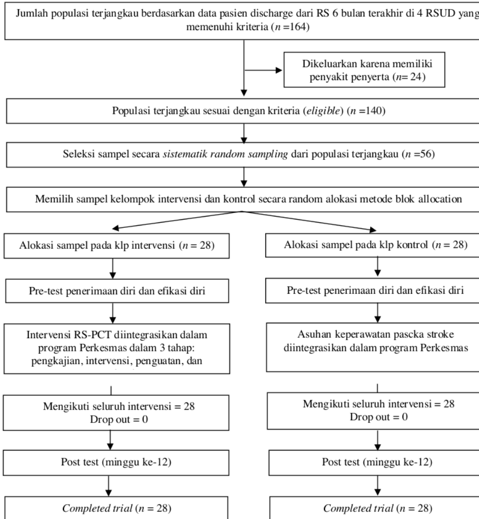
Gambar. 1 Alur Penelitian
