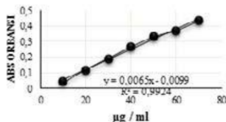
Gambar 3. Kurva Standar Quercetin
